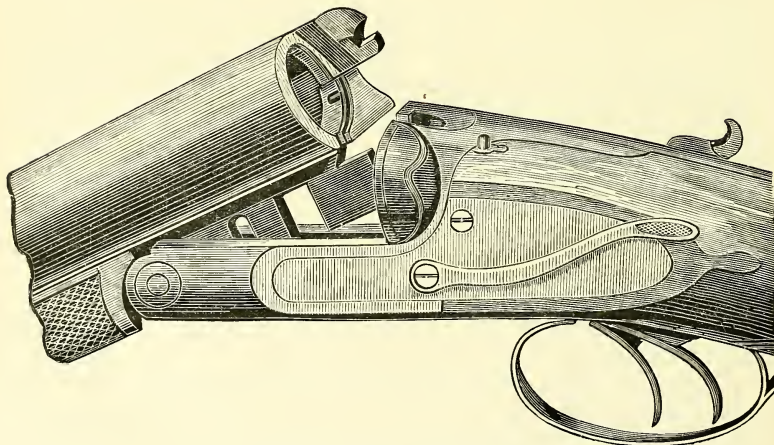
The Lefever American Hammerless Gun.
